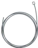
BES4WX Stainless Steel Wire Rope 1.2mmØ 49 Strand with 4x4mm Die Cast Nipple
